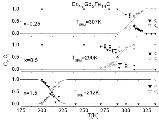
Fig. 2. The temperature dependencies of subspectra contributions for C_l — low temperature (solid triangle) and C_h — high temperature (open triangle) Zeeman sextets for \text{Er}_{2-x}\text{Gd}_x\text{Fe}_{14}\text{C} .
